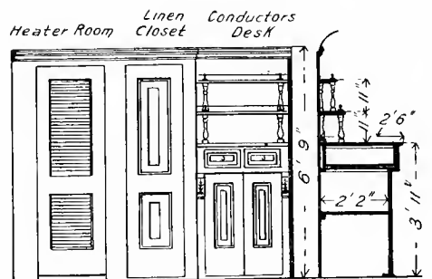
Fig. 486. Side Elevation of Conductor's Quarters.
